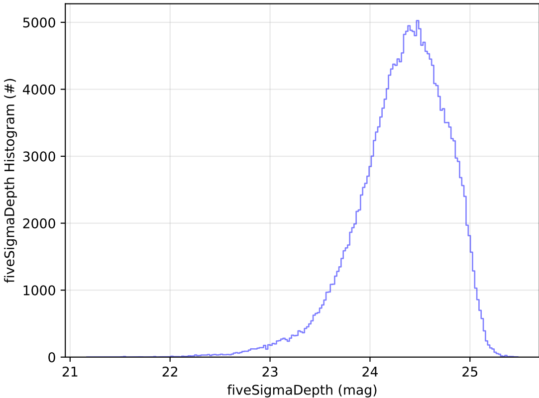
weather_cloudso18v3.5_10yrs g: fiveSigmaDepth Histogram
