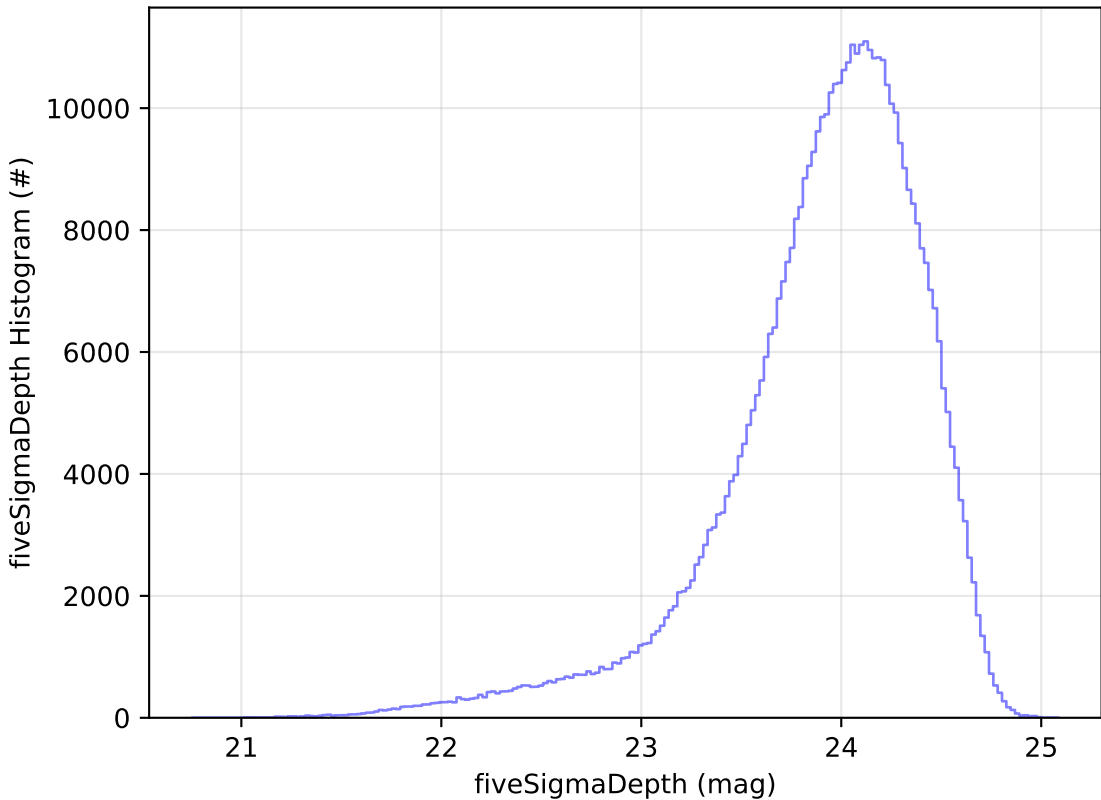
weather_cloudso18v3.5_10yrs r: fiveSigmaDepth Histogram
