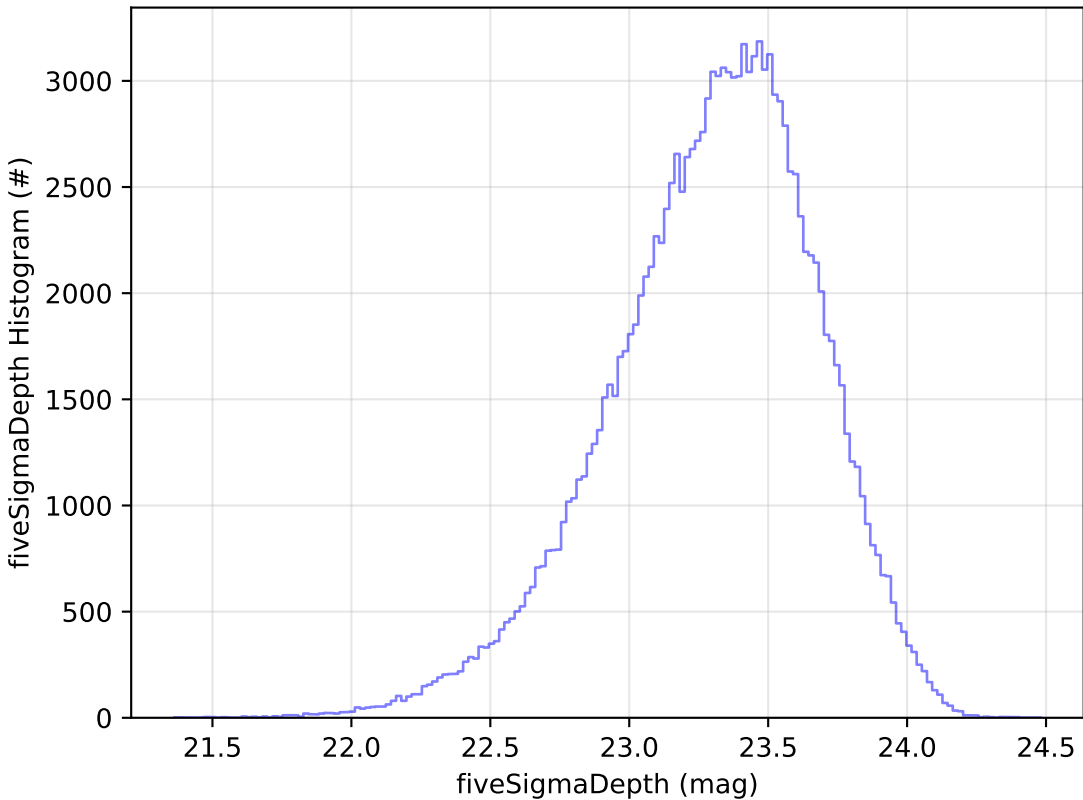
weather_cloudso18v3.5_10yrs u: fiveSigmaDepth Histogram
