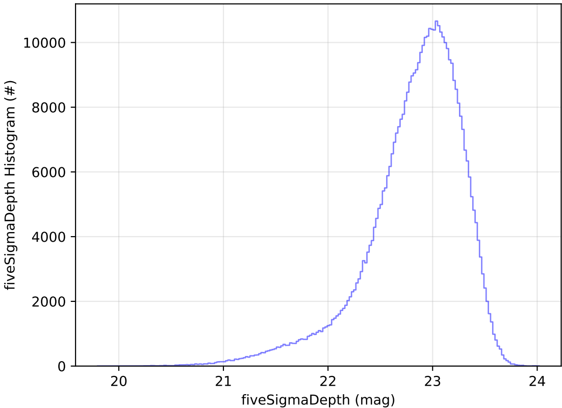
weather_cloudso18v3.5_10yrs z: fiveSigmaDepth Histogram
