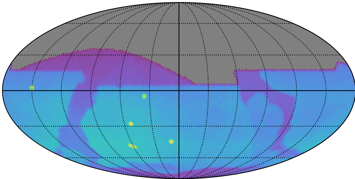
weather_cloudso1v3.5_10yrs : Brown Dwarf, L7
