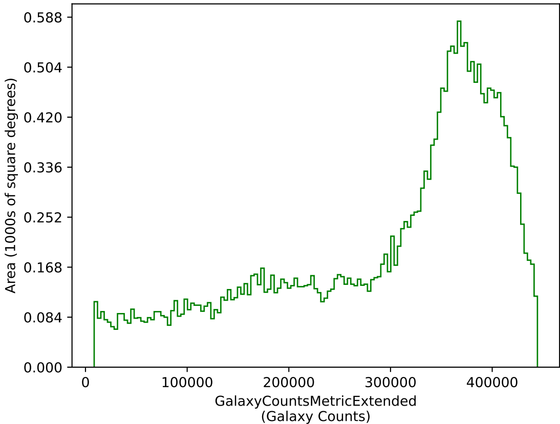
weather_cloudso1v3.5_10yrs g: GalaxyCountsMetricExtended
