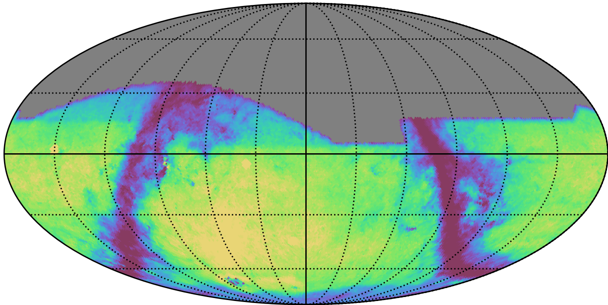
weather_cloudso1v3.5_10yrs g: GalaxyCountsMetricExtended
