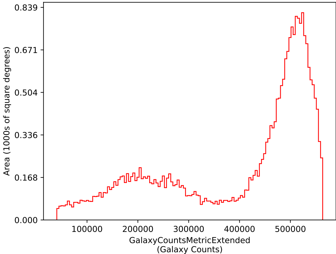
weather_cloudso1v3.5_10yrs i: GalaxyCountsMetricExtended
