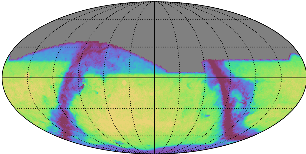
weather_cloudso1v3.5_10yrs i: GalaxyCountsMetricExtended
