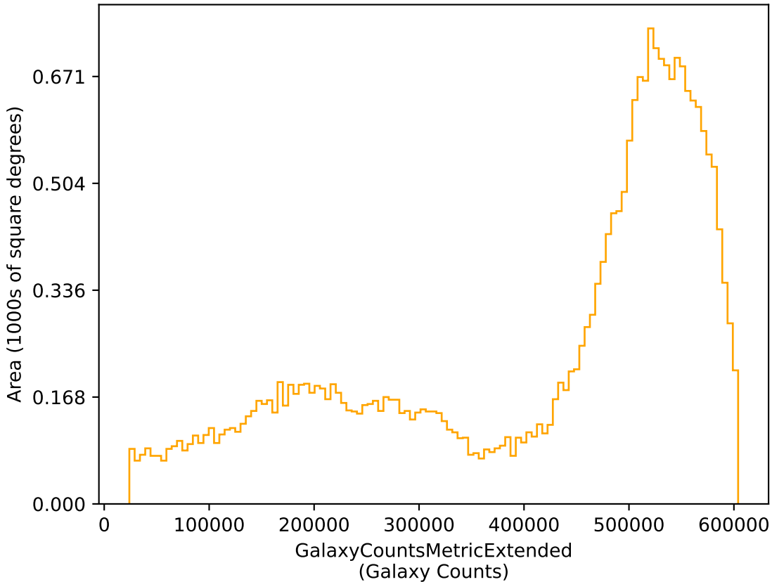
weather_cloudso1v3.5_10yrs r: GalaxyCountsMetricExtended
