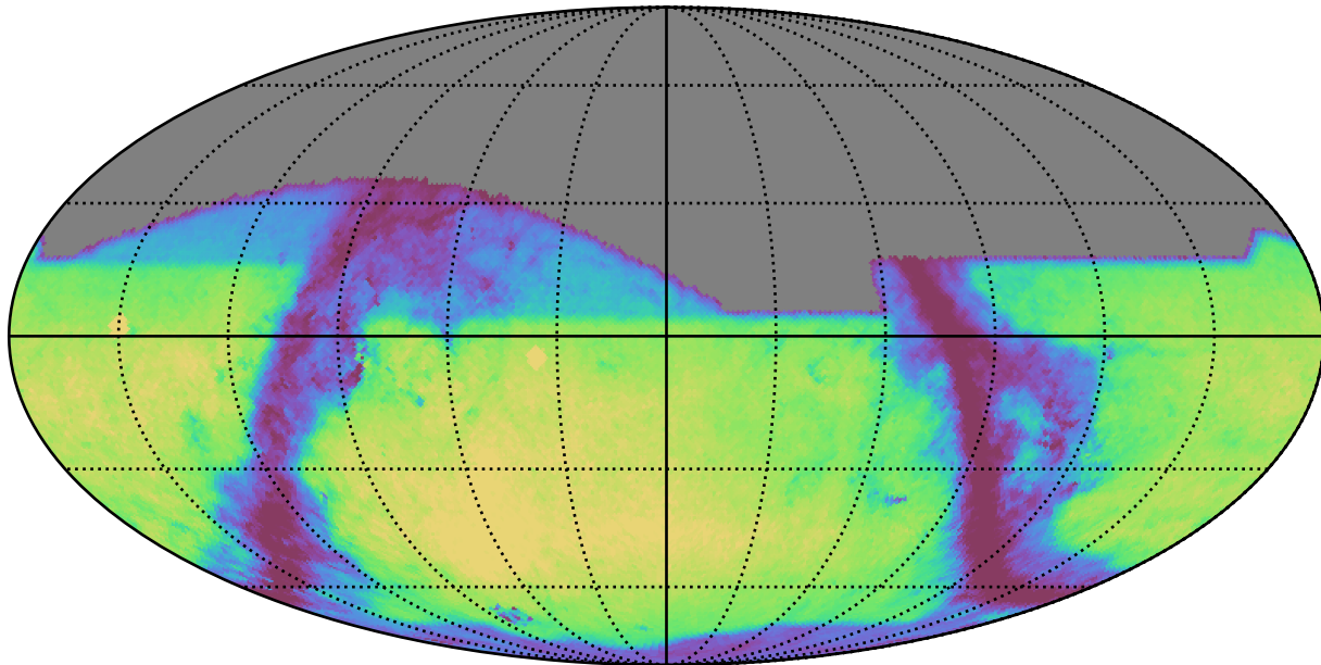
weather_cloudso1v3.5_10yrs r: GalaxyCountsMetricExtended
