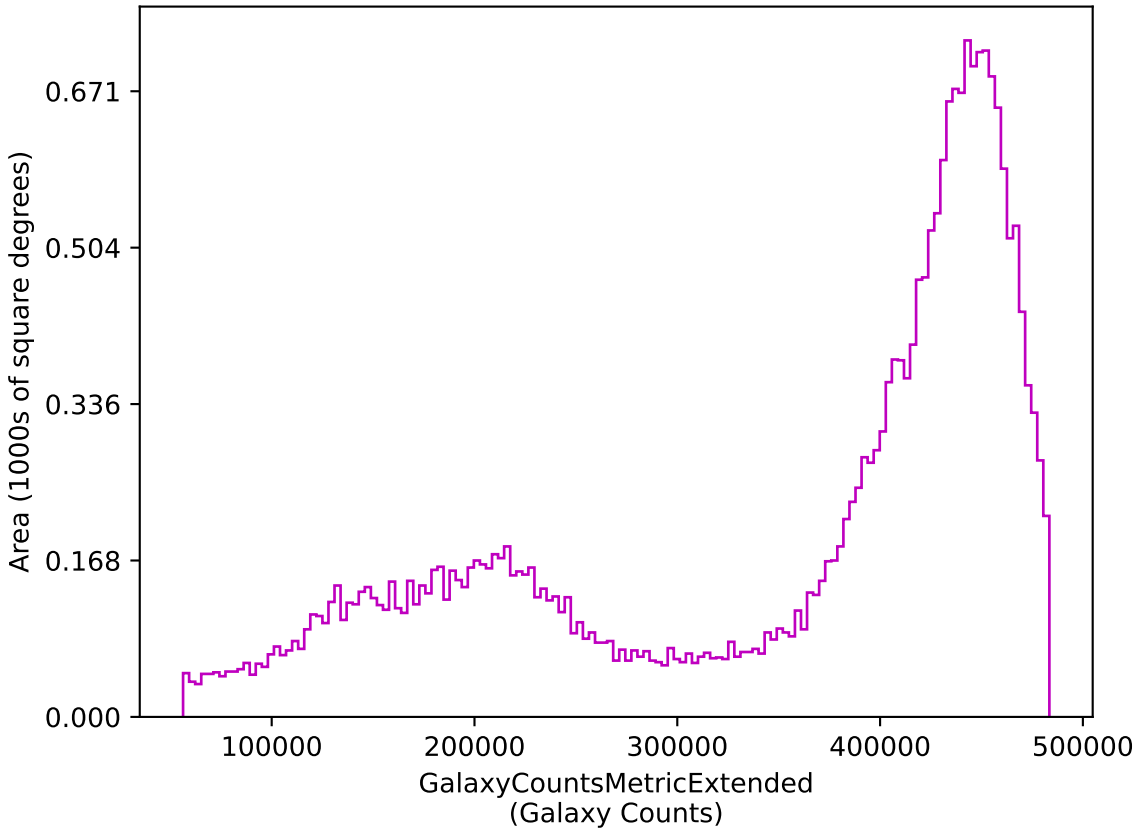
weather_cloudso1v3.5_10yrs z: GalaxyCountsMetricExtended
