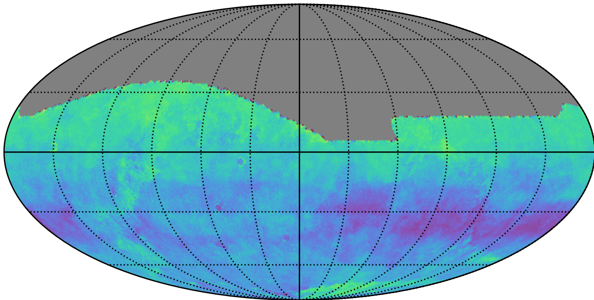
weather_cloudso1v3.5_10yrs r: Kuiper rotSkyPos
