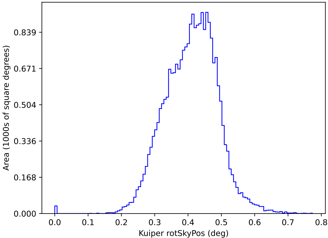
weather_cloudso1v3.5_10yrs y: Kuiper rotSkyPos
