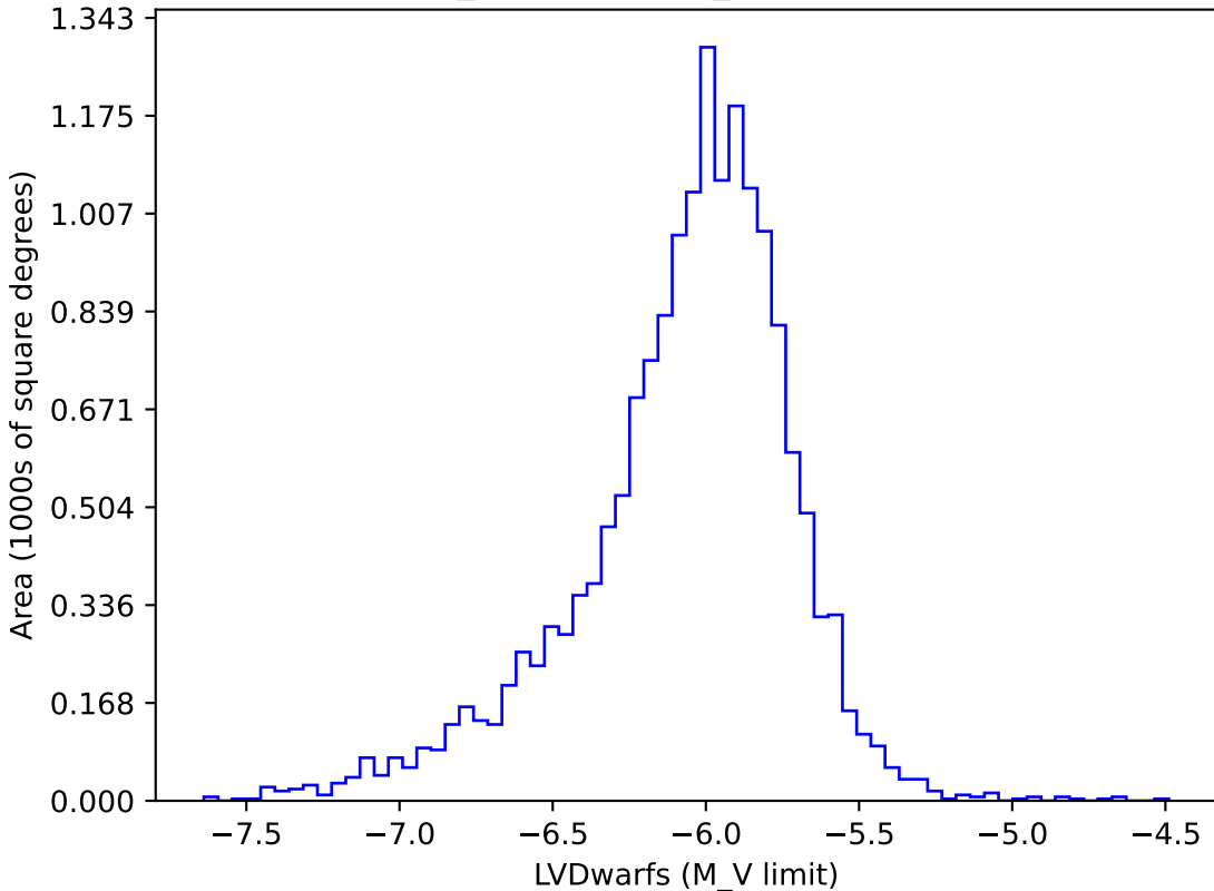
weather_cloudso1v3.5_10yrs gi: LVDwarfs
