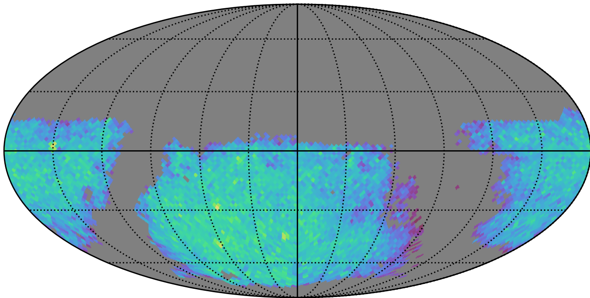
weather_cloudso1v3.5_10yrs gi: LVDwarfs
