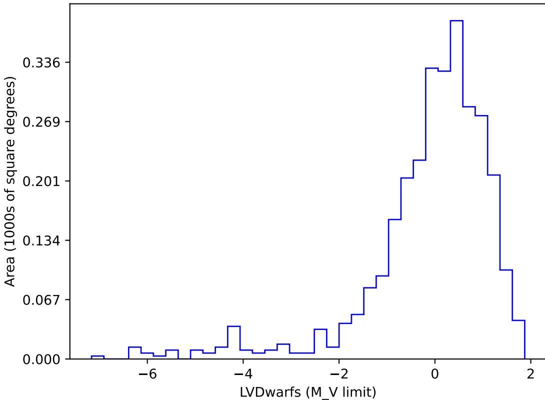
weather_cloudso1v3.5_10yrs gi SCP: LVDwarfs
