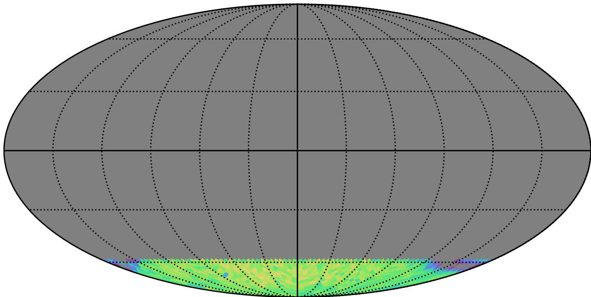
weather_cloudso1v3.5_10yrs gi SCP: LVDwarfs
