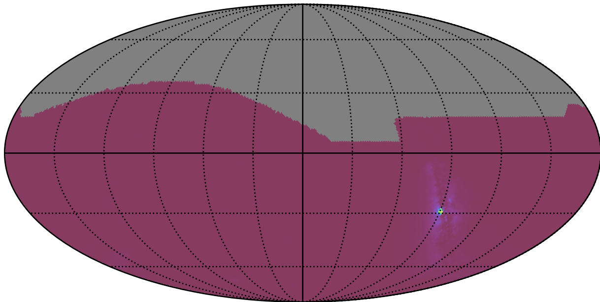
weather_cloudso1v3.5_10yrs : NlcPoints
