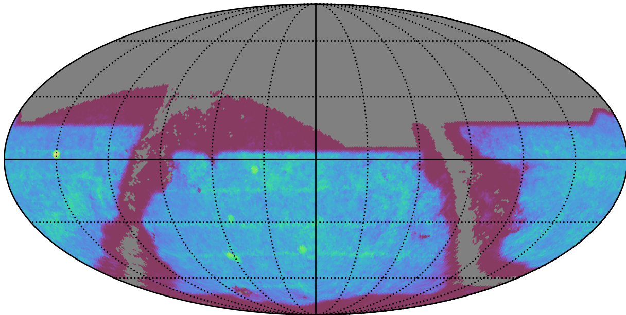
weather_cloudso1v3.5_10yrs : SNSLMetric
