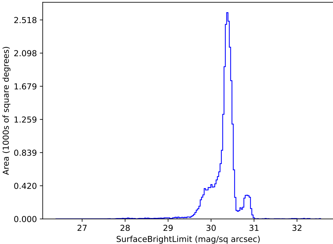
weather_cloudso1v3.5_10yrs g: SurfaceBrightLimit
