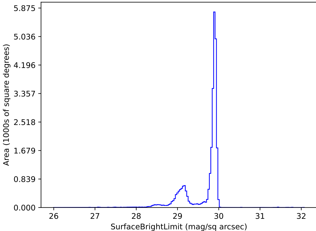
weather_cloudso1v3.5_10yrs i: SurfaceBrightLimit
