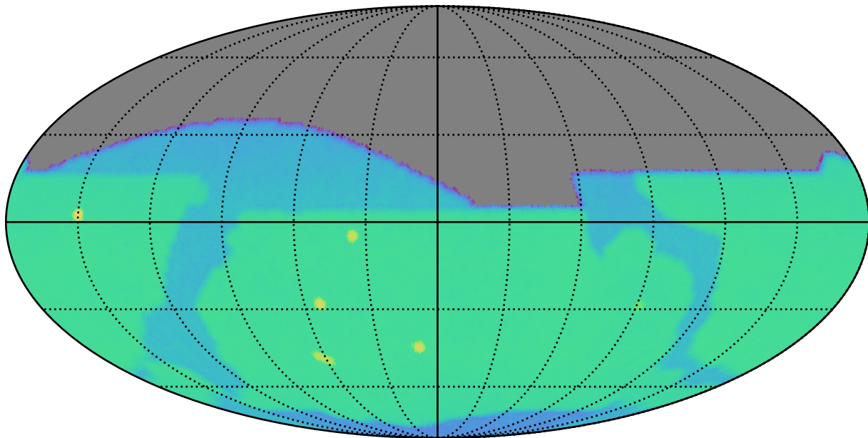
weather_cloudso1v3.5_10yrs i: SurfaceBrightLimit
