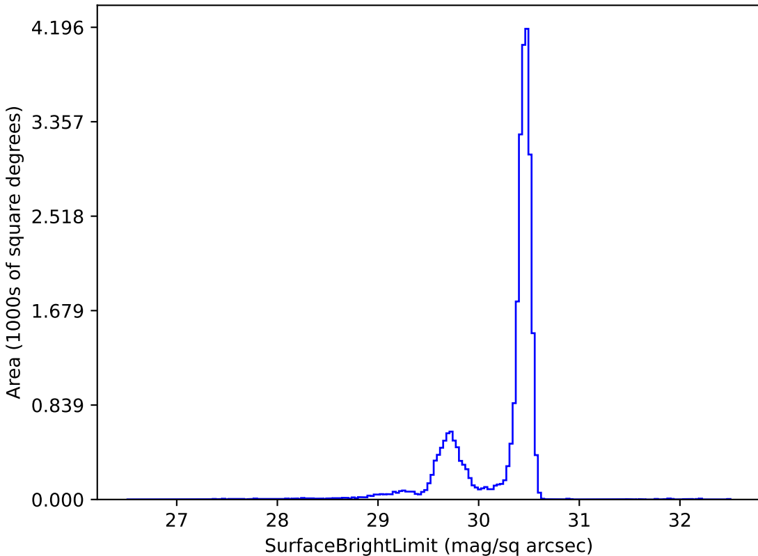
weather_cloudso1v3.5_10yrs r: SurfaceBrightLimit
