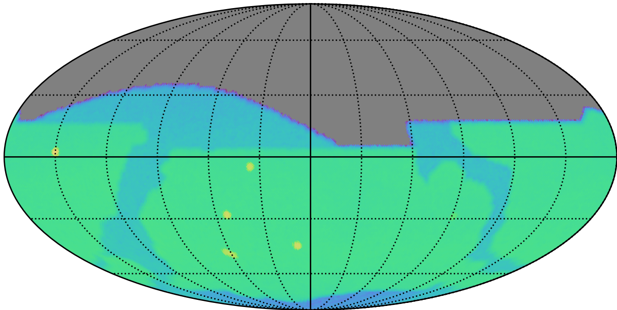
weather_cloudso1v3.5_10yrs r: SurfaceBrightLimit
