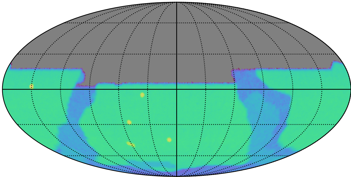
weather_cloudso1v3.5_10yrs y: SurfaceBrightLimit
