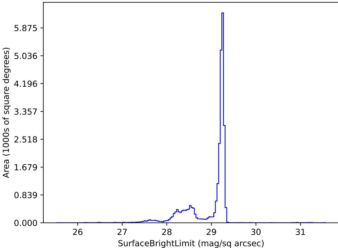
weather_cloudso1v3.5_10yrs z: SurfaceBrightLimit
