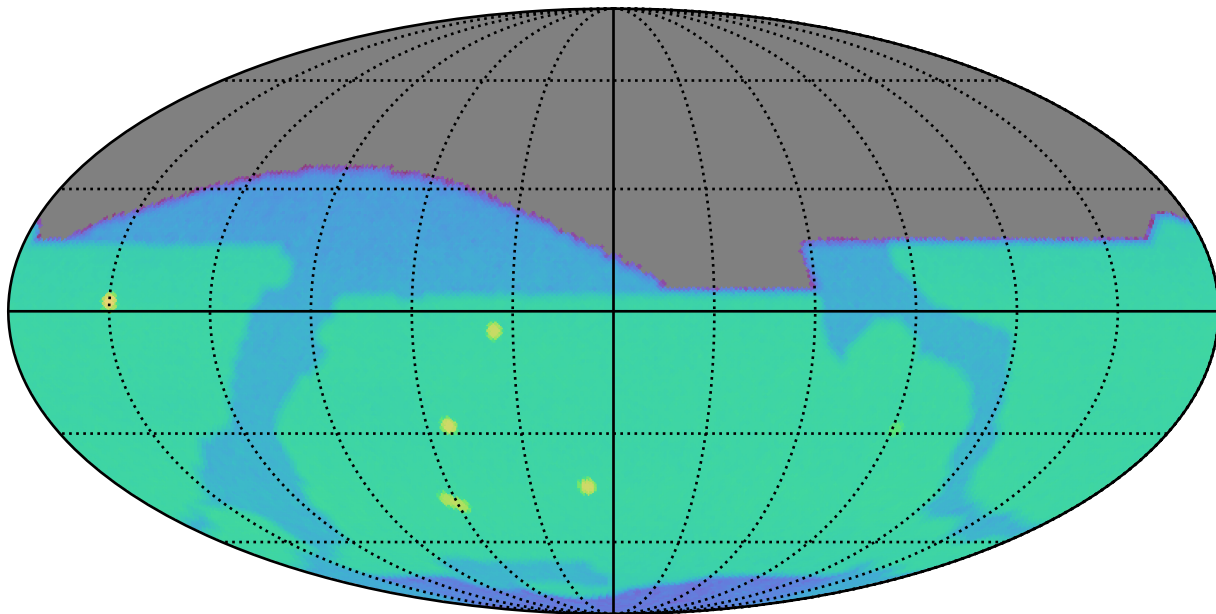
weather_cloudso1v3.5_10yrs z: SurfaceBrightLimit
