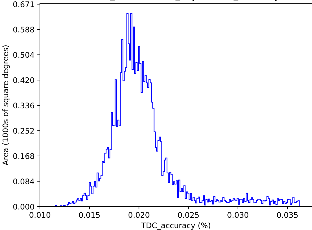
weather_cloudso1v3.5_10yrs : TDC_accuracy
