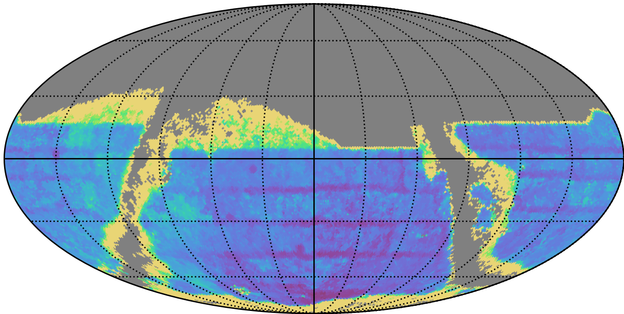
weather_cloudso1v3.5_10yrs : TDC_accuracy
