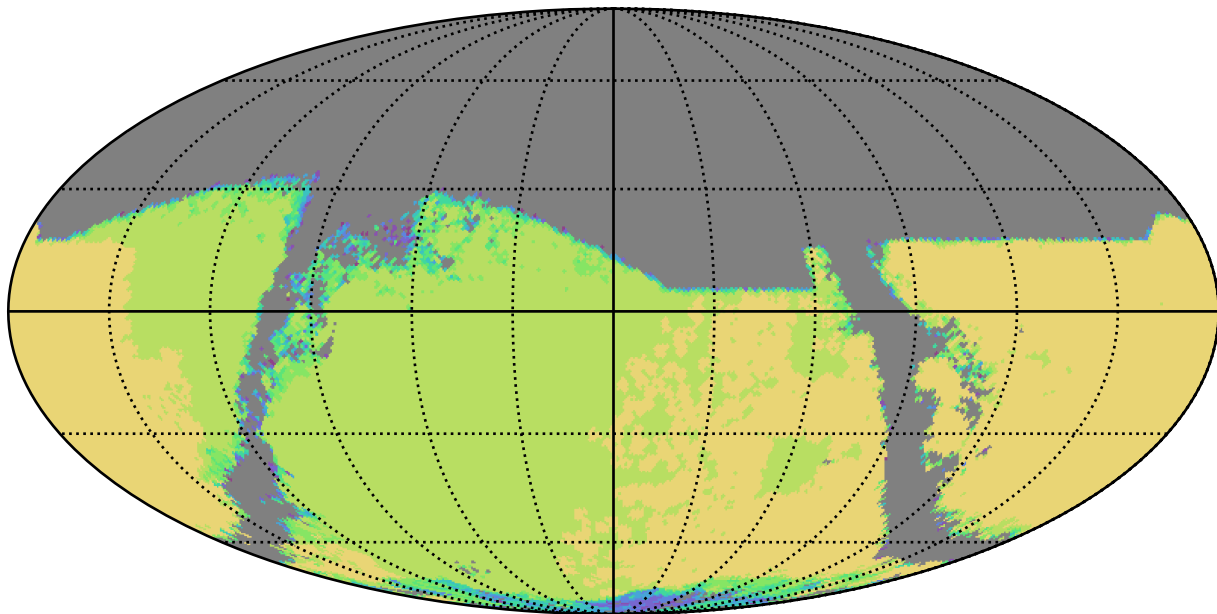
weather_cloudso1v3.5_10yrs : TDC_campaign
