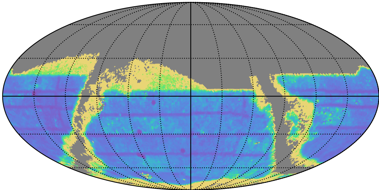
weather_cloudso1v3.5_10yrs : TDC_precision
