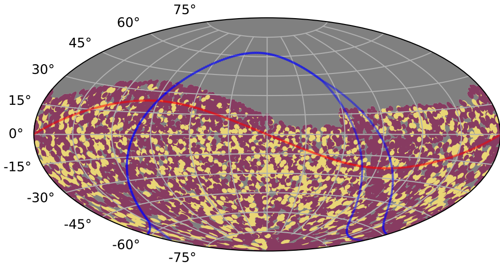
weather_cloudso1v3.5_10yrs : TDEsPopMetric_prepeak
