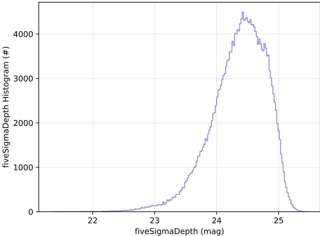
weather_cloudso1v3.5_10yrs g: fiveSigmaDepth Histogram
