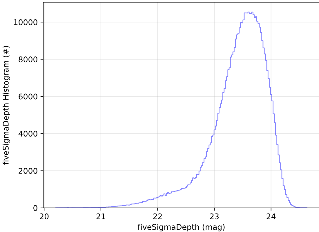
weather_cloudso1v3.5_10yrs i: fiveSigmaDepth Histogram
