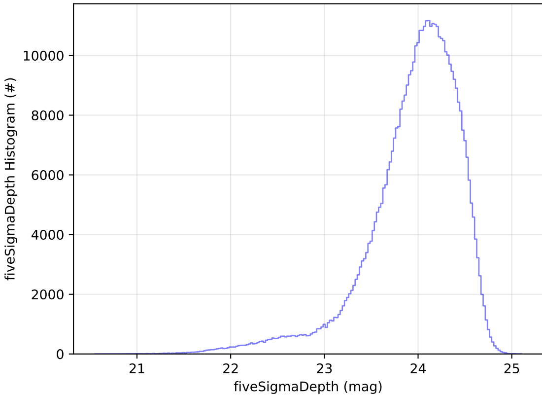
weather_cloudso1v3.5_10yrs r: fiveSigmaDepth Histogram
