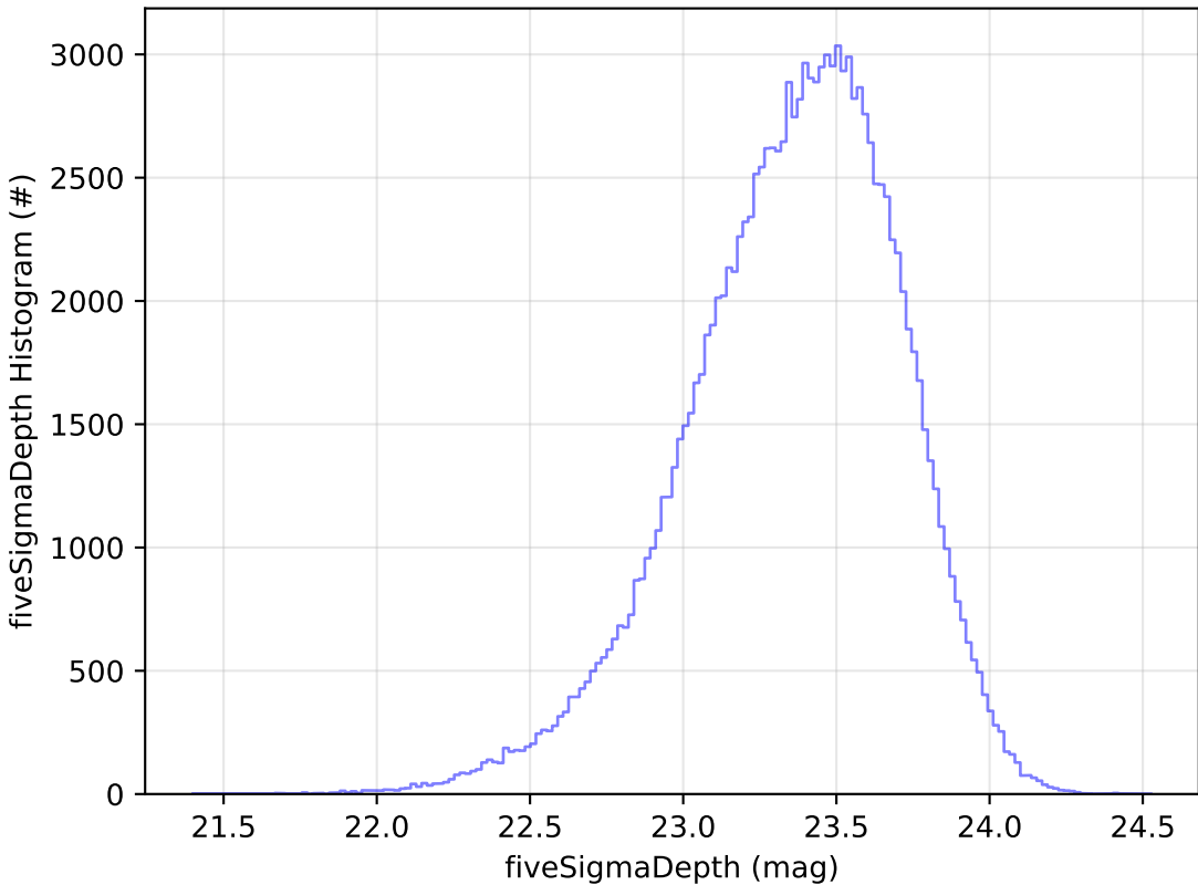
weather_cloudso1v3.5_10yrs u: fiveSigmaDepth Histogram
