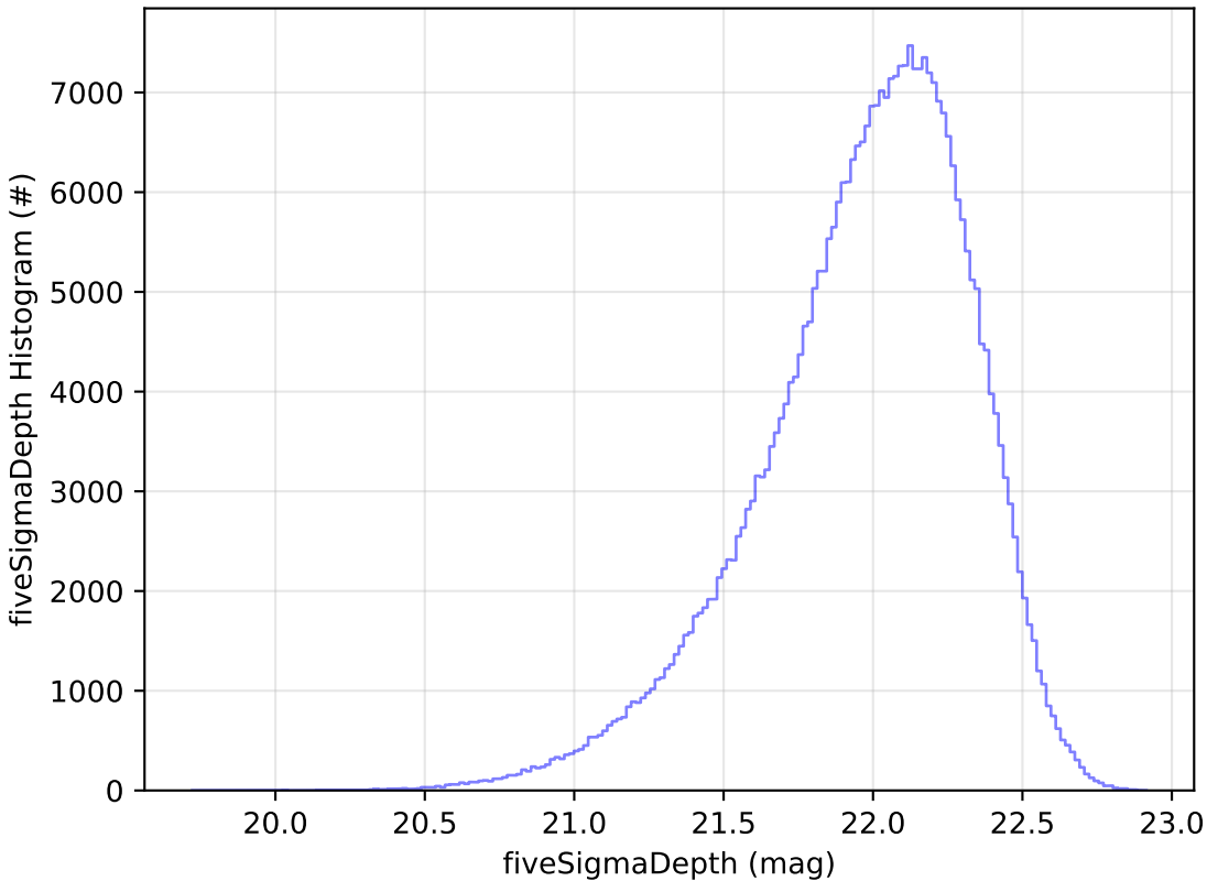
weather_cloudso1v3.5_10yrs y: fiveSigmaDepth Histogram
