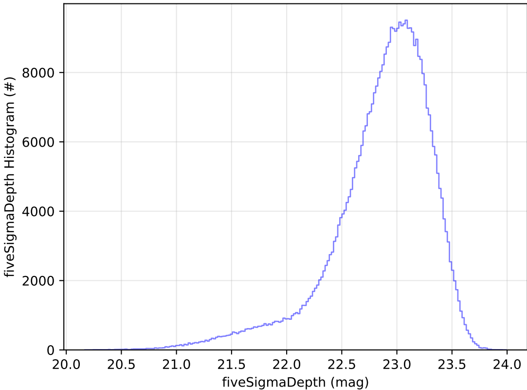
weather_cloudso1v3.5_10yrs z: fiveSigmaDepth Histogram
