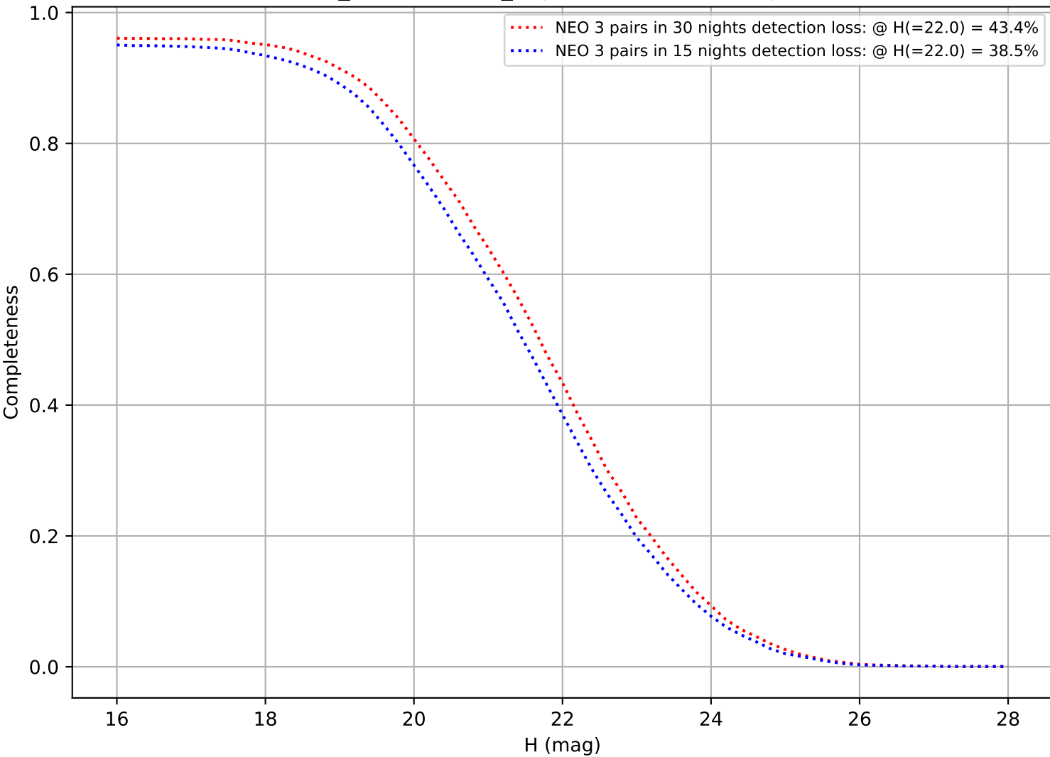
weather_cloudso1v3.5_10yrs: DifferentialCompleteness
