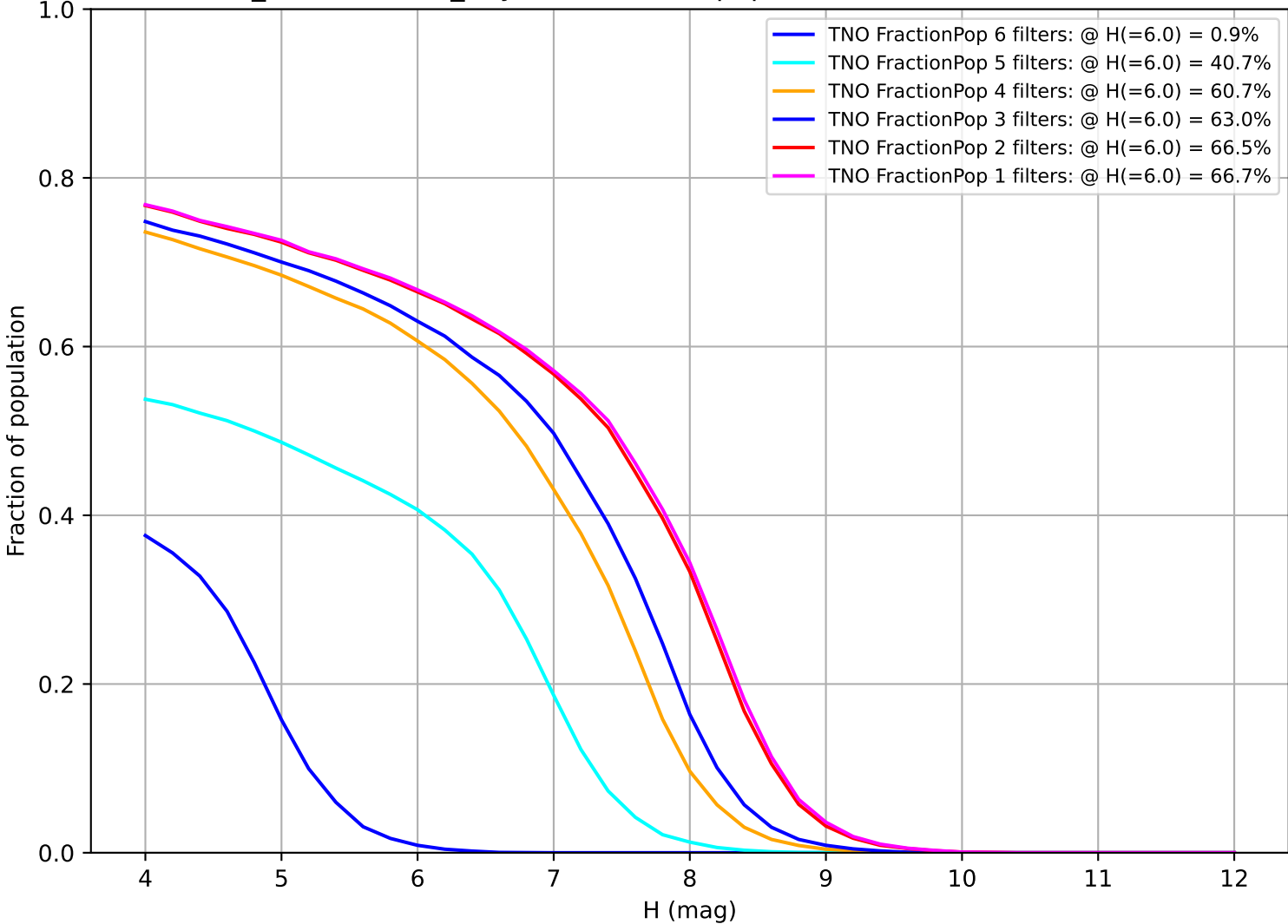
weather_cloudso1v3.5_10yrs: Fraction of population with colors in X filters TNO
