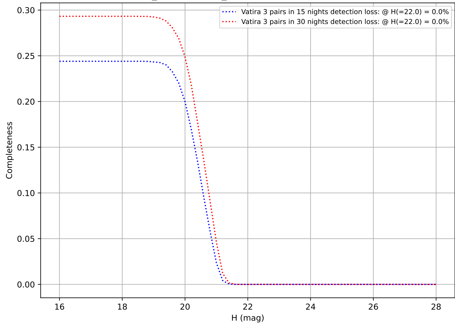
weather_cloudso1v3.5_10yrs: DifferentialCompleteness
