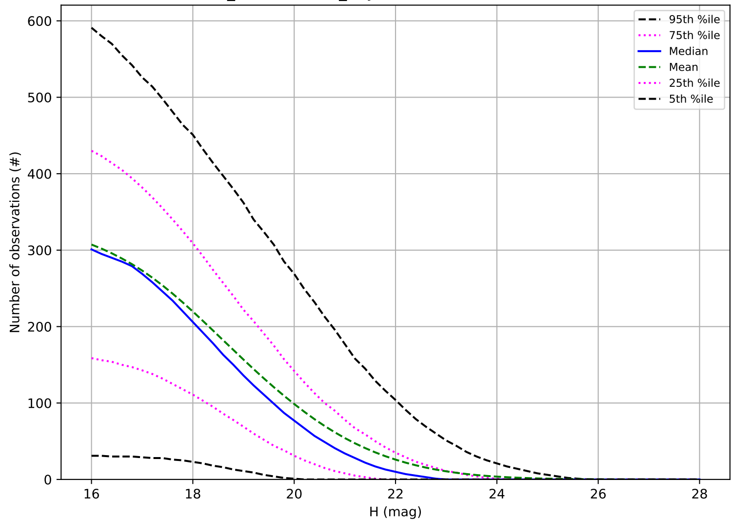
weather_cloudso1v3.5_10yrs: Number of observations NEO
