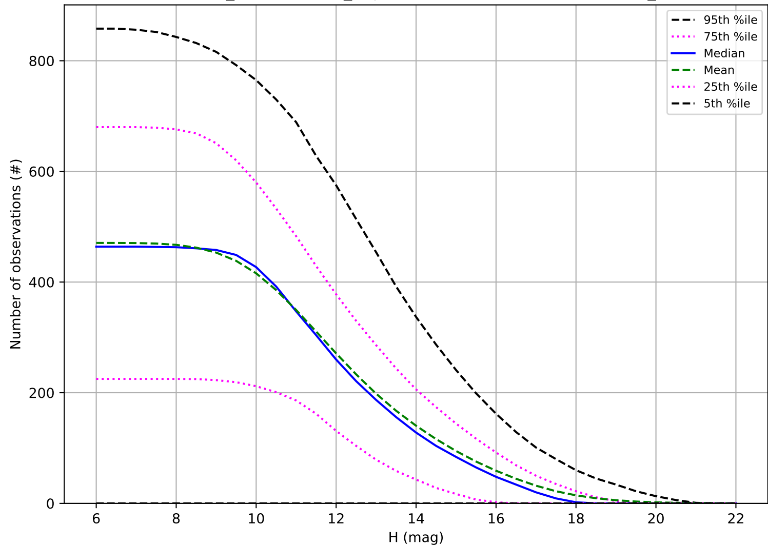
weather_cloudso1v3.5_10yrs: Number of observations OCC_r5
