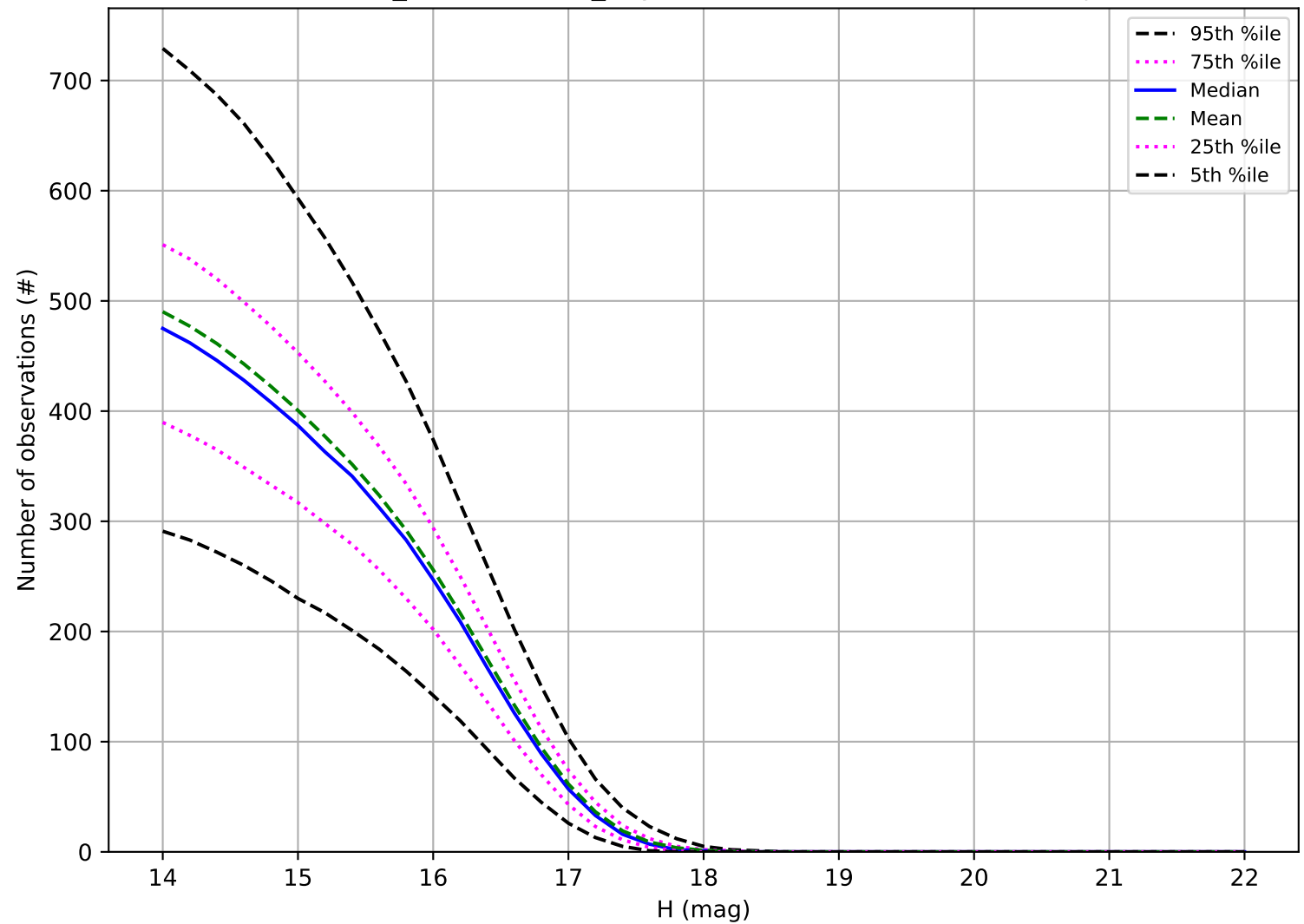
weather_cloudso1v3.5_10yrs: Number of observations Trojan
