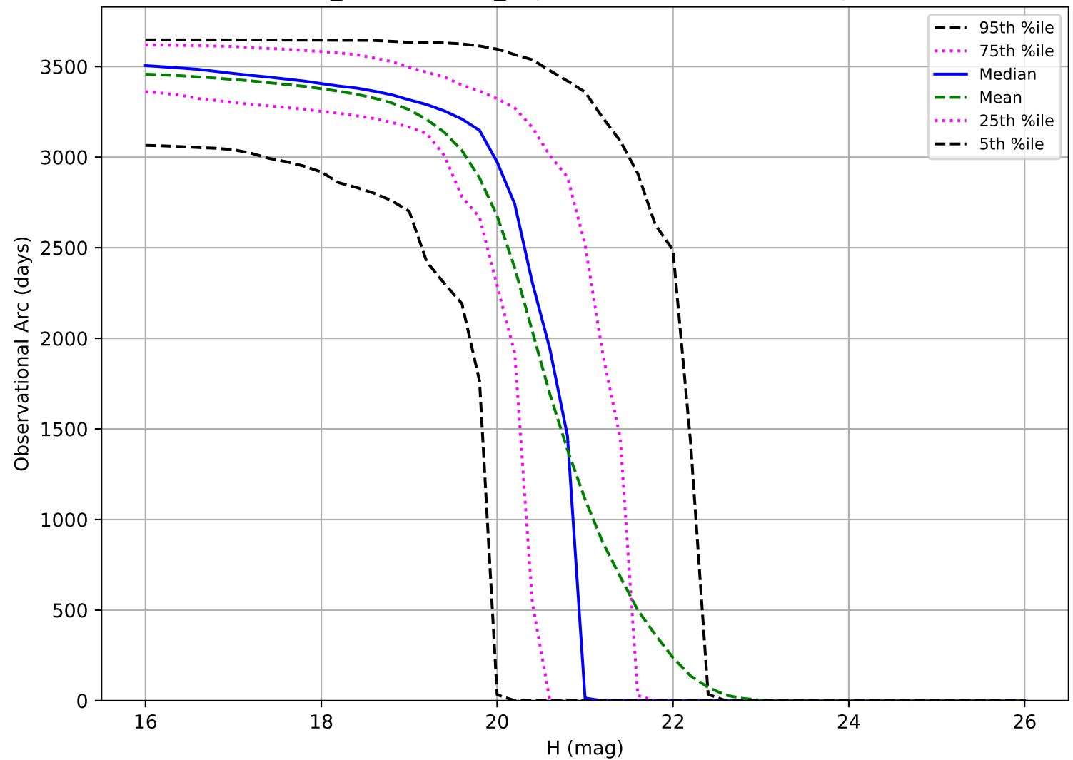
weather_cloudso1v3.5_10yrs: Observational Arc Length MBA
