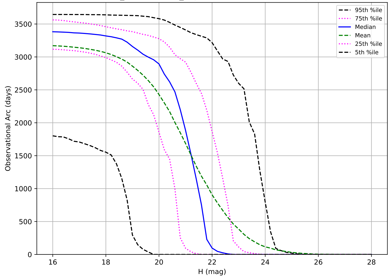
weather_cloudso1v3.5_10yrs: Observational Arc Length NEO
