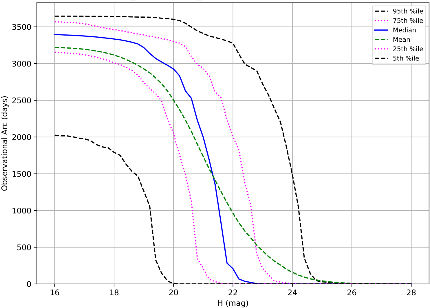
weather_cloudso1v3.5_10yrs: Observational Arc Length PHA
