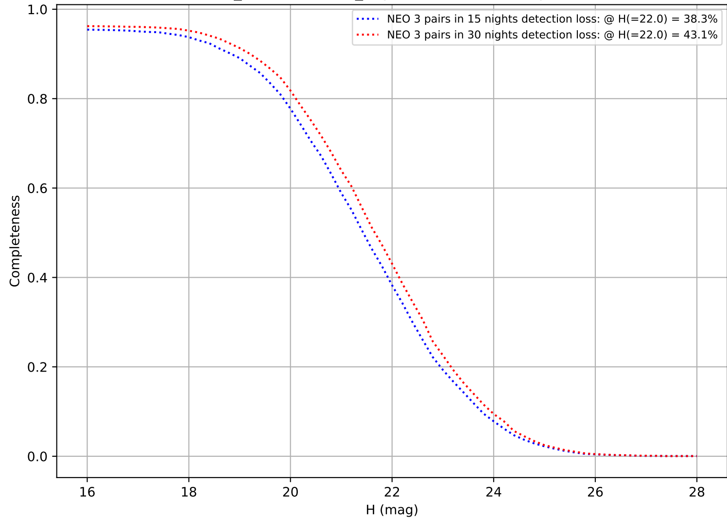
weather_cloudso20v3.5_10yrs: DifferentialCompleteness
