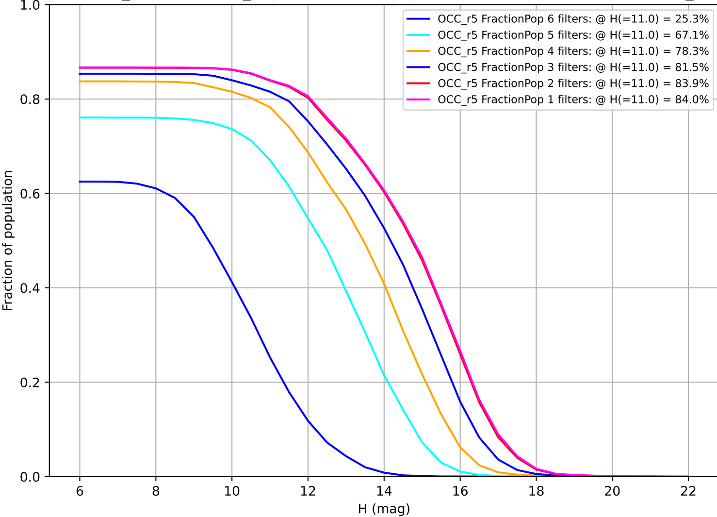
weather_cloudso20v3.5_10yrs: Fraction of population with colors in X filters OCC_r5
